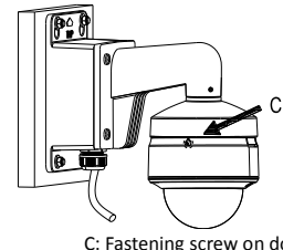
C: Fastening screw on dome
